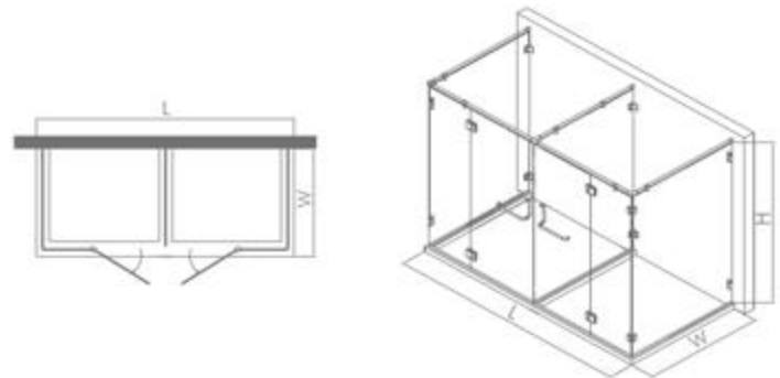
KDLLHE00172 Standard:1100x2200x1100x2000mm Customization:L: 1900-2500mm W:800-1300mm H: 1850-2200mm
