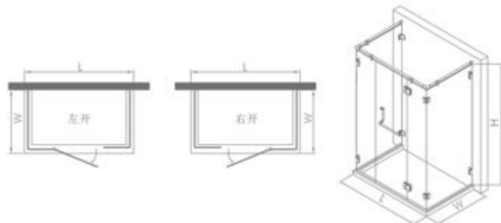
KDLLHU00151 Standard:900x1500x2000mm Customization:L: 1200-1600mm W:800-1300mm H: 1850-2200mm
